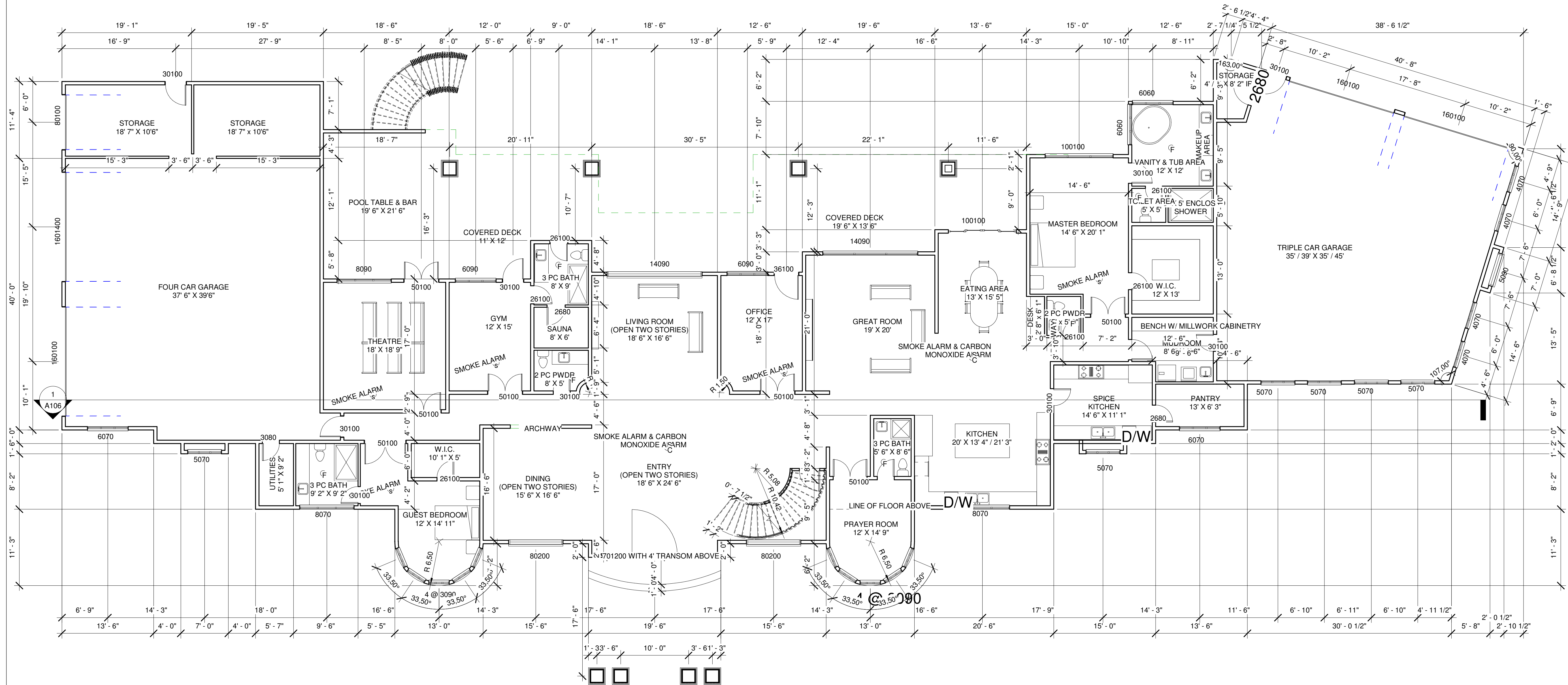
1 MAIN FLOOR 1/8" = 1'-0"
