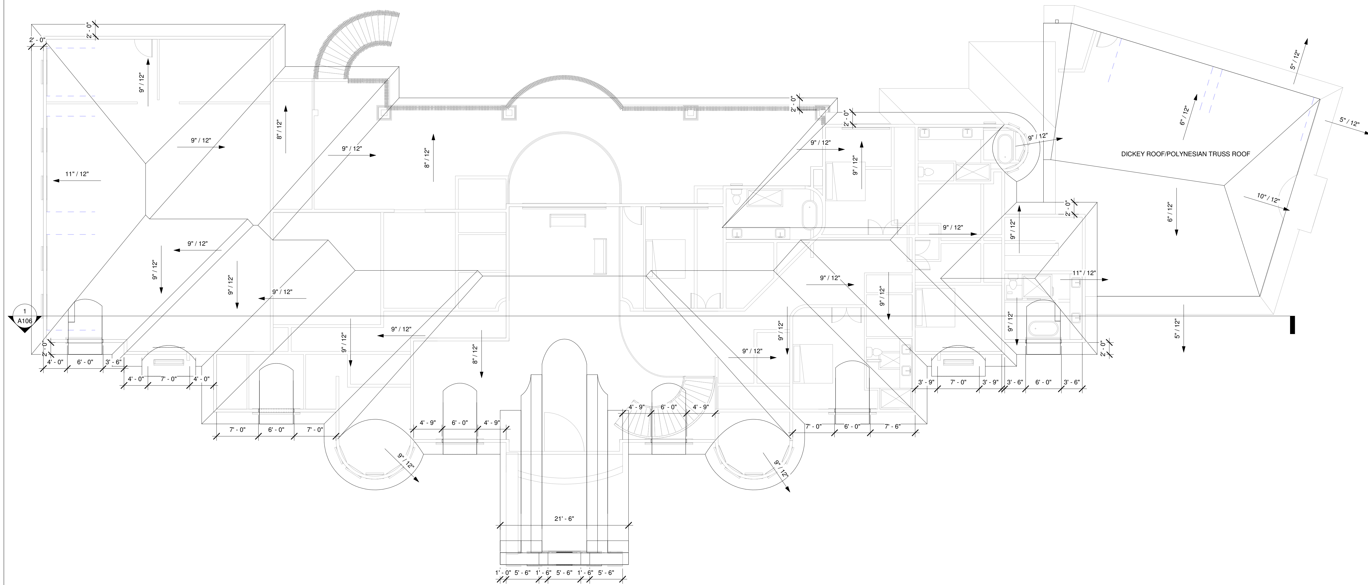
3 ROOF PLATE 1/8" = 1'-0"
