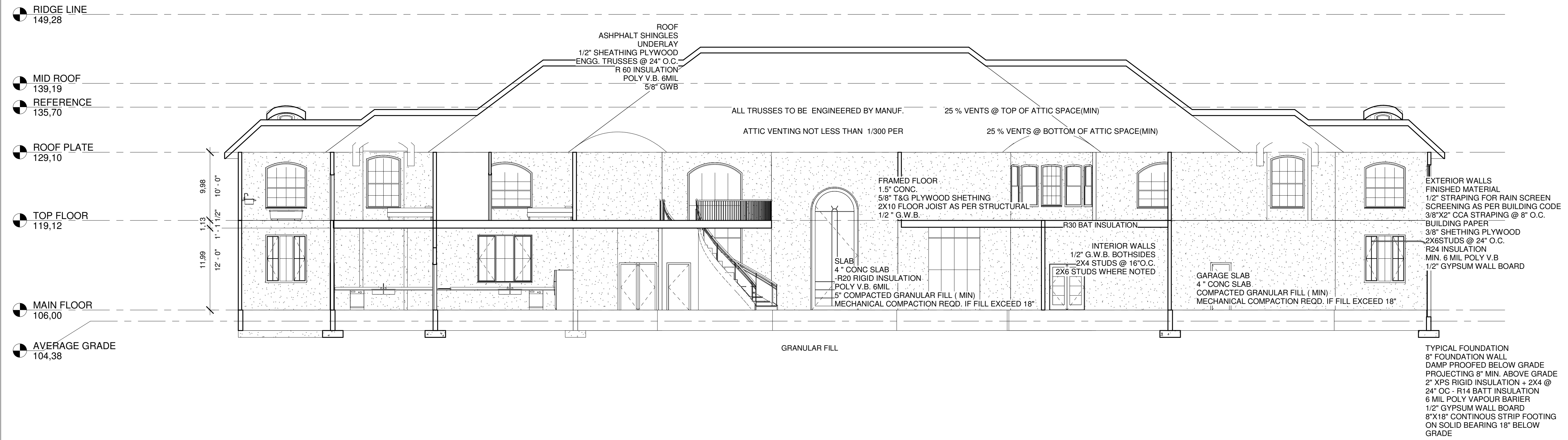
1 Section 3 1/8" = 1'-0"
